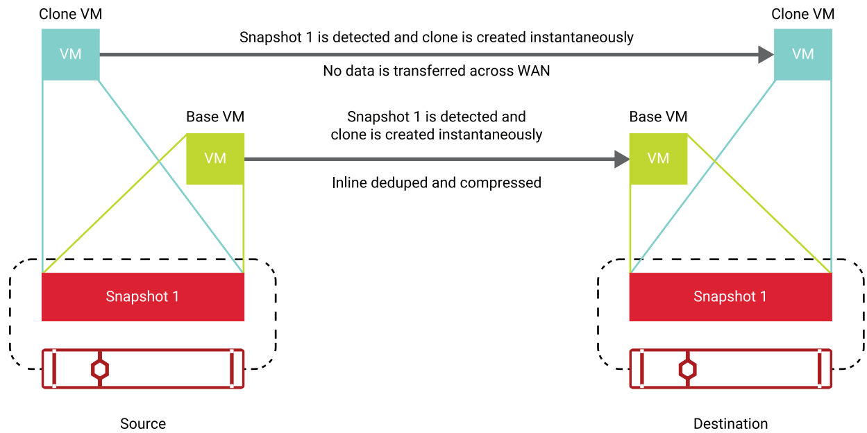
Figure 2. Flexible, instant VM cloning
